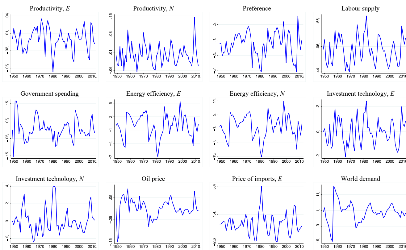
Figure 2. Residuals
