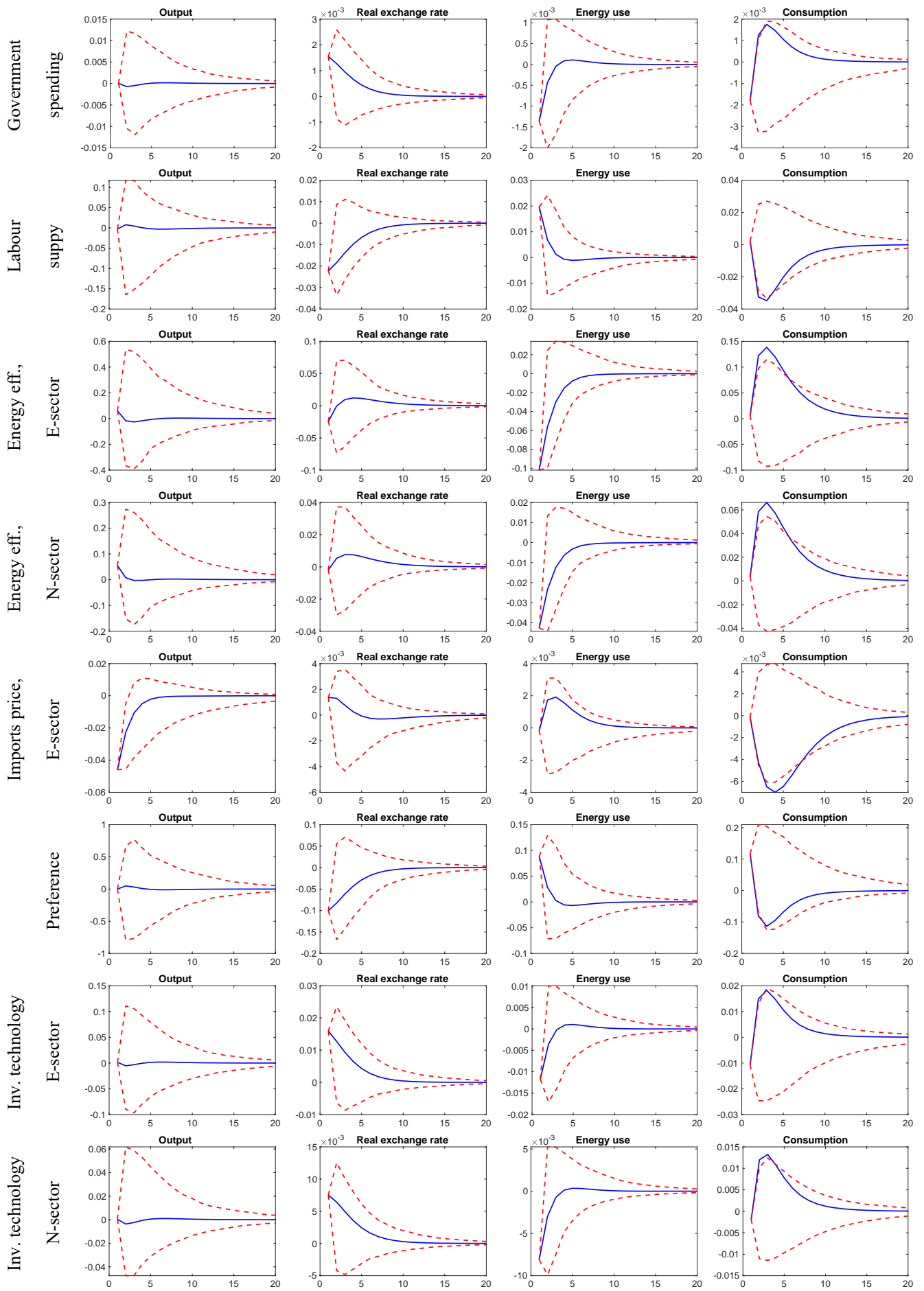
Figure D1. Additional VAR impulse response functions
