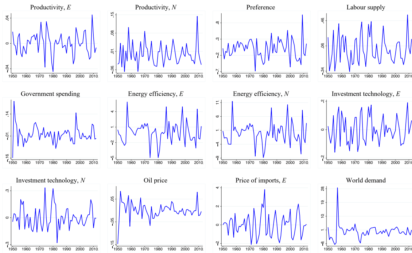
Figure 3. Shocks
