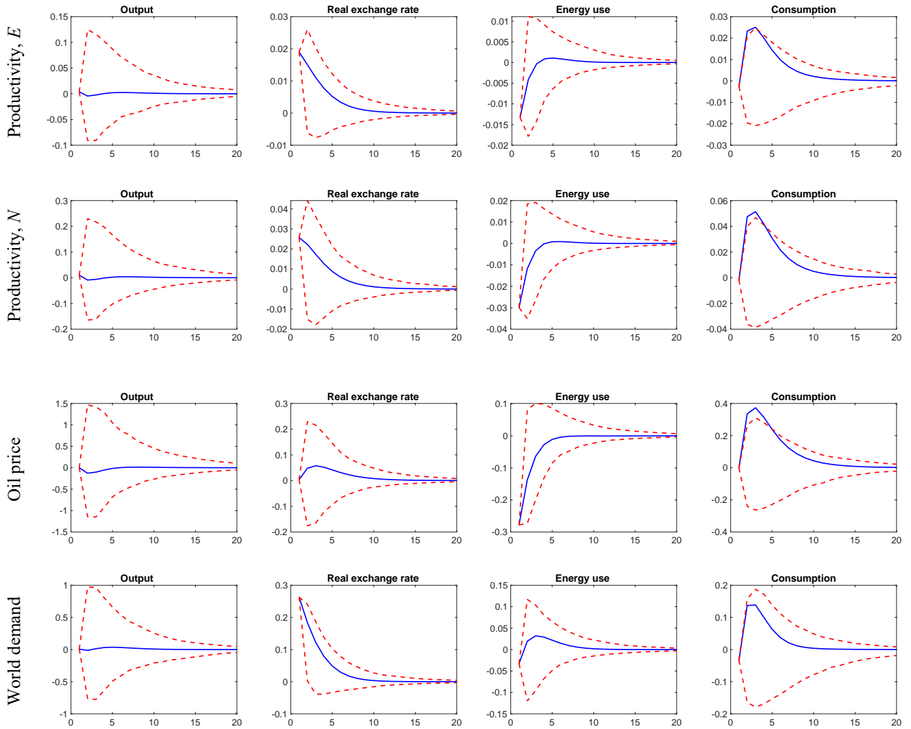
Figure 4. VAR impulse response functions
