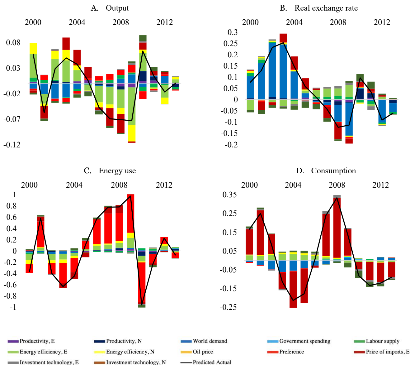
Figure 5. Historical decompositions of macro variables in the VAR
